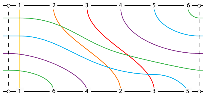
Figure 10: Unrolling of a circular line diagram representing the circular permutation (1, 6, 4, 2, 3, 5)
