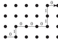
Fig. 2. Path encoded by the word w = 01000110 .
