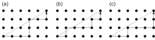
Fig. 5. Given \Phi(0) = -1 and \Phi(1) = +1 , three paths coded by words from the set C_{-1/4} . The word in (c) is also in B_{-1/4} while in (a) the prefix 00011 \in C_{-1/5} and in (b) the prefix 01 \in C_0 .
