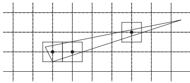
Fig. 1. The discretization of a continuous object resulting in a non-connected set.
