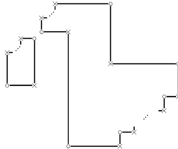
Fig. 4.1. Planar representation of (\nu', \mu) .
